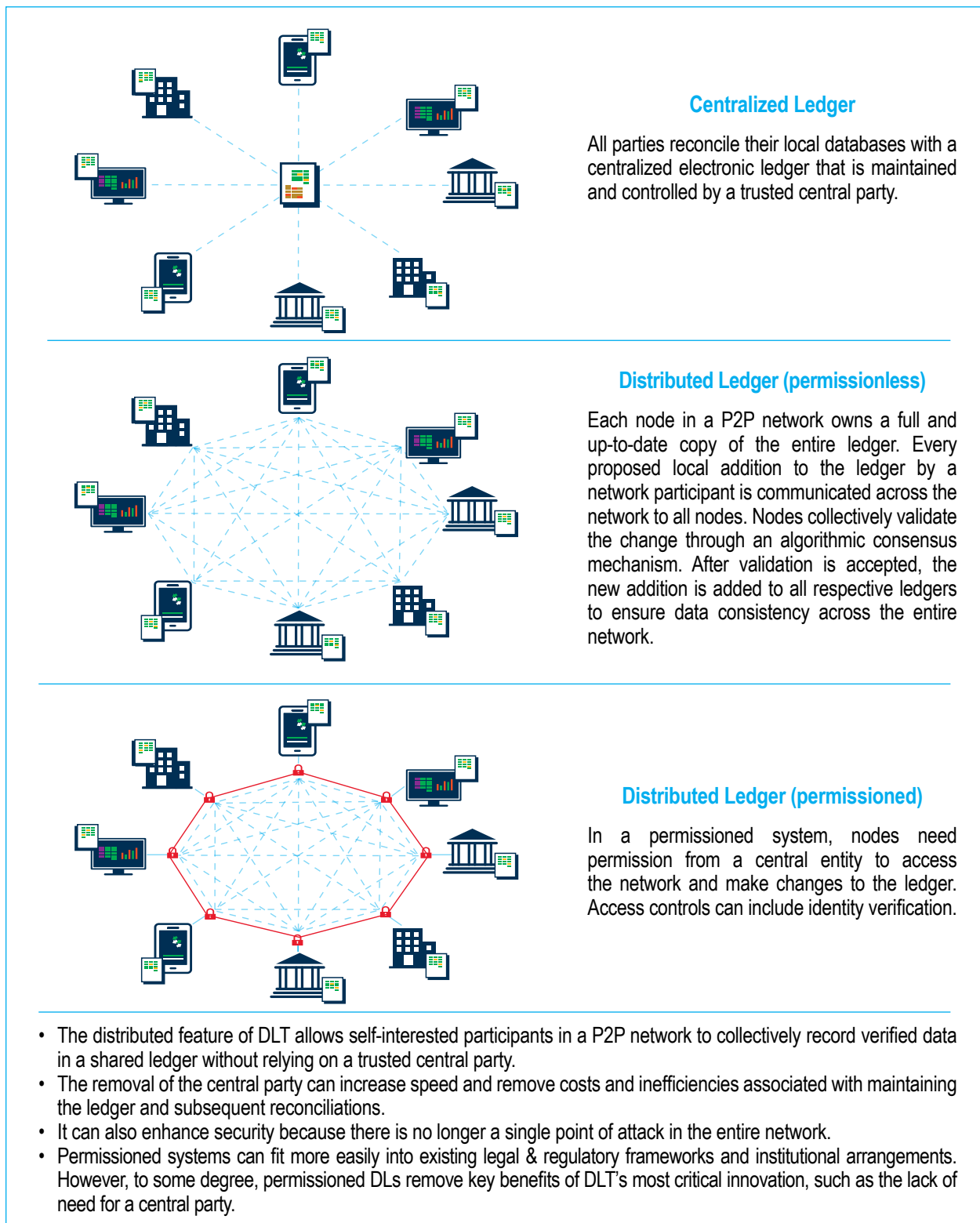
Figure 2: Distributed Ledger
