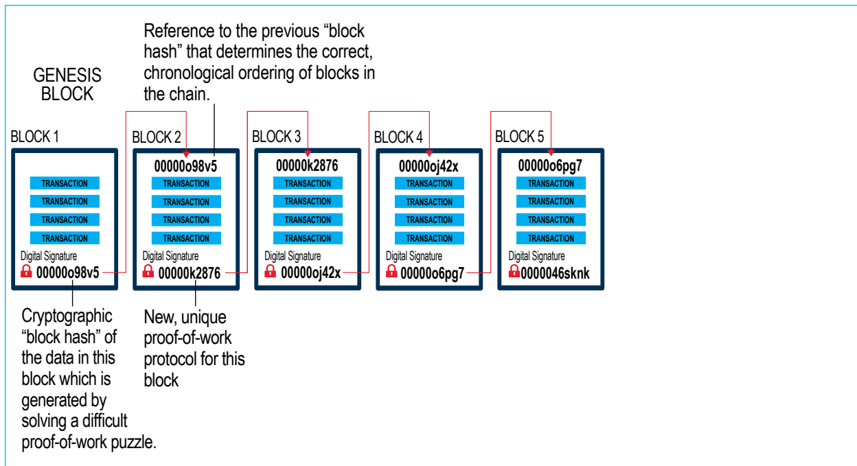
Figure 4: Blockchain Structure
