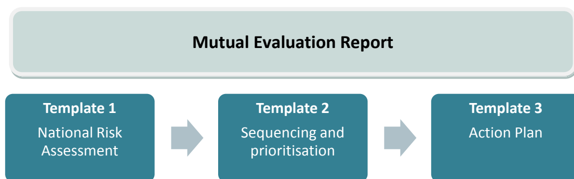
Figure 3. SIP framework
